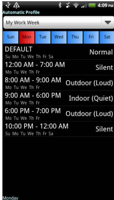
Automatic Profiles
