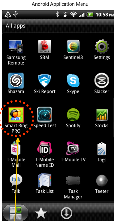
Program Icon
